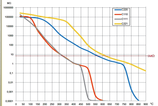
Insulation resistance variation curves of terminal blocks as a function of temperature, made in different types of ceramic, (C110, C111, C220, C221), in thickness 2mm. The value of 5MΩ is the normative limit.
