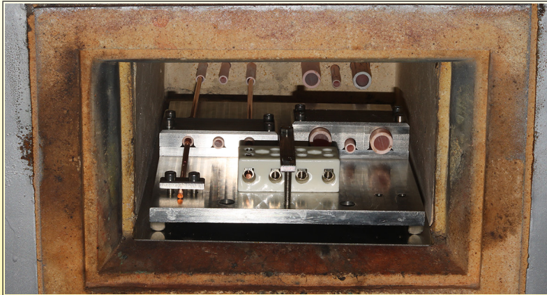
Test oven for the resistivity of ceramics as a function of temperature (Ultimheat Laboratory)
