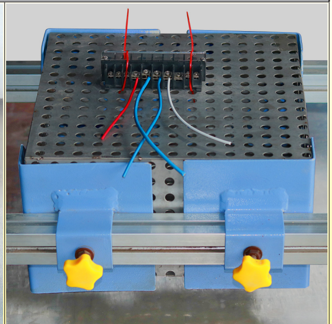
Connection block during test
