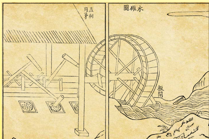
Waterwheel and trip-hammer (水確 shui dui) for grinding minerals (Tiangong Kaiwu, Song Yingxing 1637)
